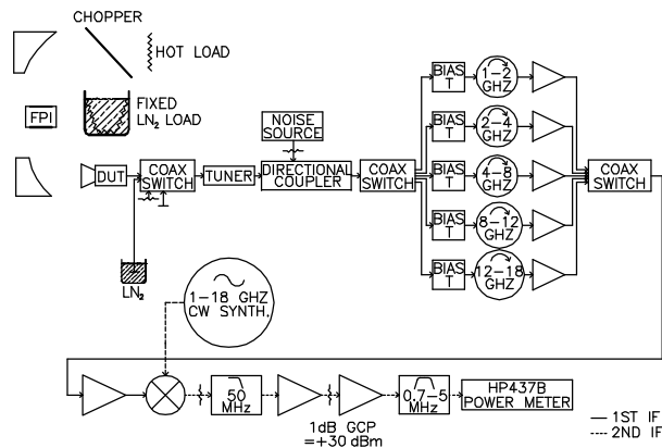
Fig. 2: Block diagram of test system IF section
