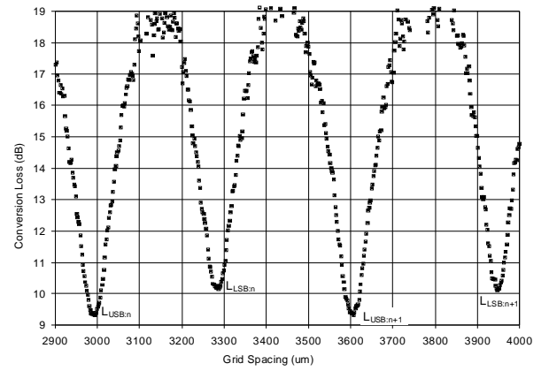
Fig. 5: mixer conversion loss as a function of FPI grid spacing
